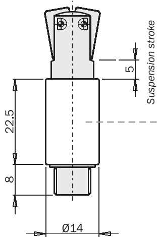
Gripper + Suspension
