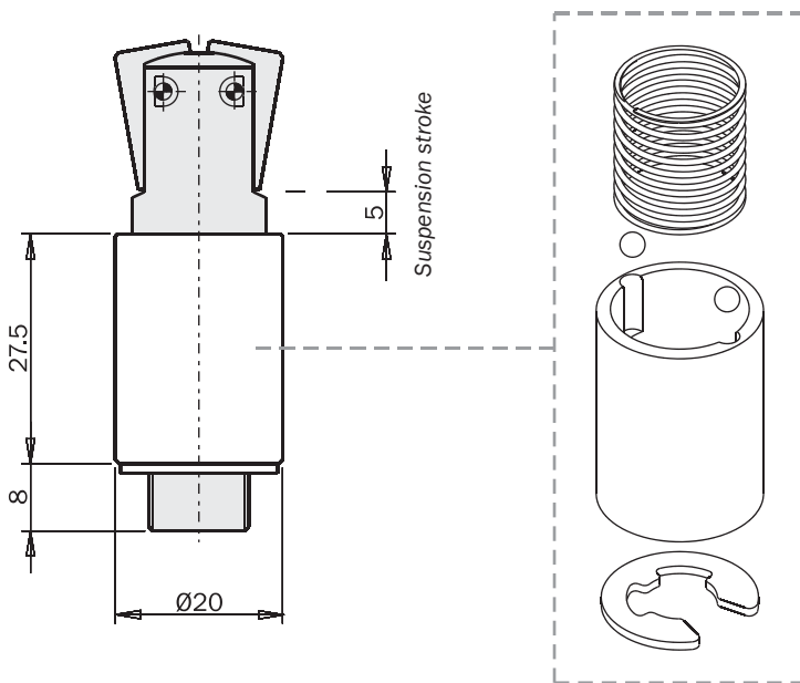
Gripper + Suspension
