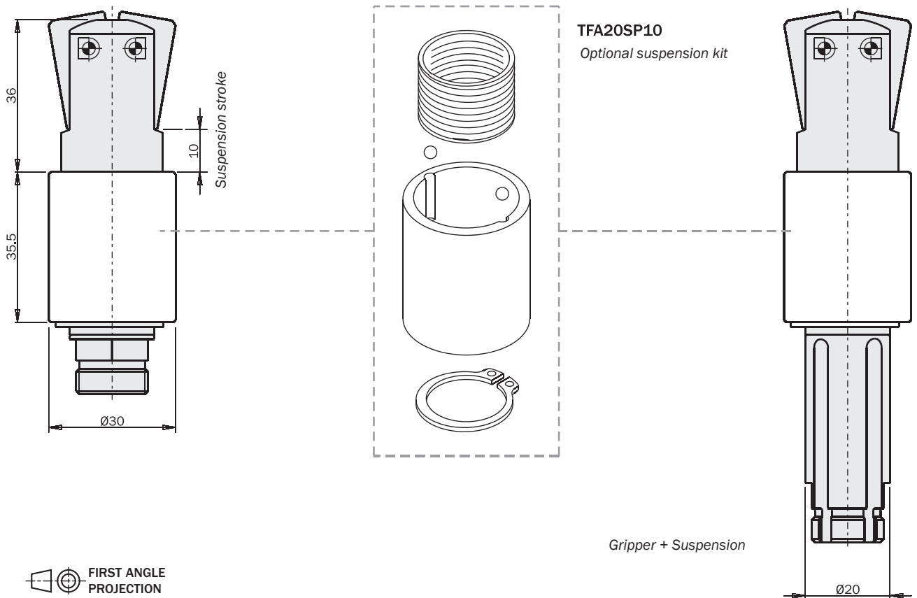
Gripper + Suspension
